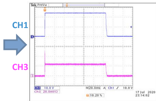
IN and OUT signal in current sinking circuit, CH1 = IN, CH3 = I_{OUT} \times 10\Omega .
