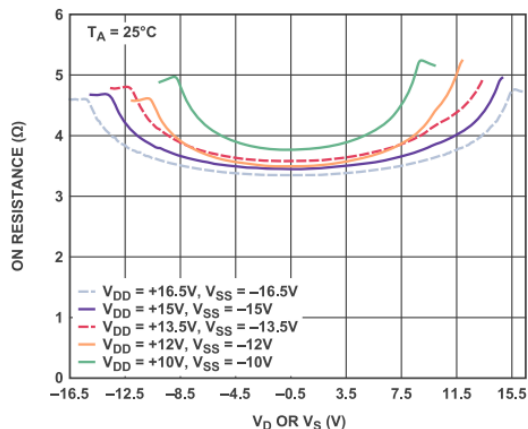
On Resistance vs. V D or V S for a Dual Supply
