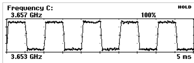
Figure 2: Pulse modulated frequency or FSK
