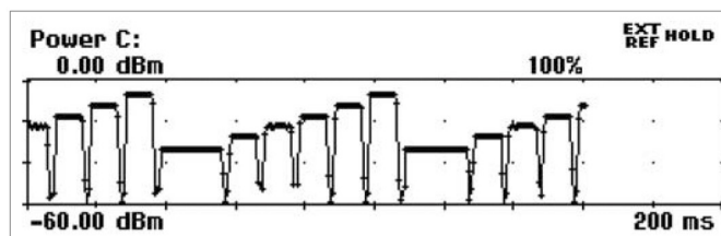
Figure 6: Power step from generator (-30 to -5dBm in 5dBm steps) NOTE: output is turned off shortly betw. power steps
