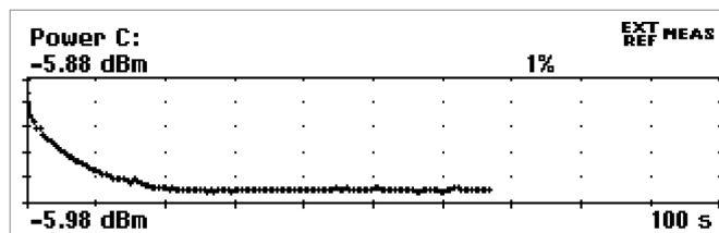
Figure 3: Generator start-up power settling
