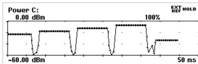
Figure 7: Power step (close up)
