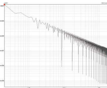
Figure 5: ADEV vs (Zero-dead-time measurement) reveals poor performance of a synthesised function generator
