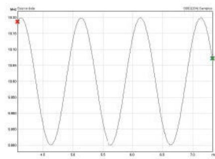
Figure 4: 10 MHz with 1kHz FM -Modulation domain view.
