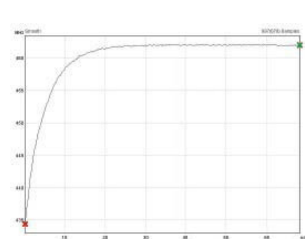
Figure 9: Frequency settling of VCO after step change of input voltage.
