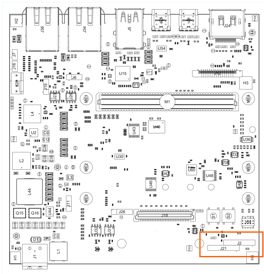
Figure 4: Location of J2 and J21 Headers on Board
