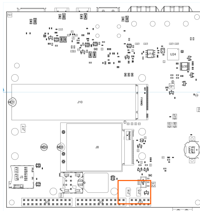
Figure 3: Location of CAN bus 1 (J14) and CAN bus 2 (J15)
