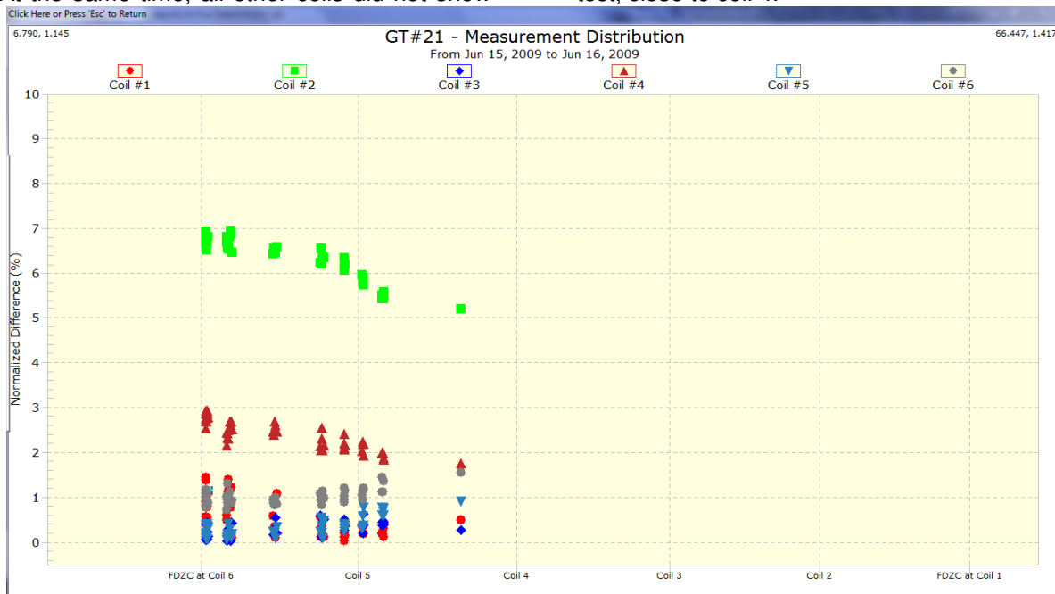
Fig. 5: X-axis is FDZC position on rotor, Y-axis is the normalized flux difference from pole A to pole
