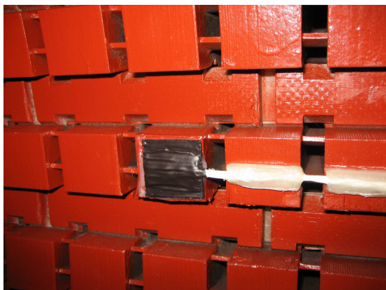
Fig 1: New probe design shown mounted on a stator core tooth
