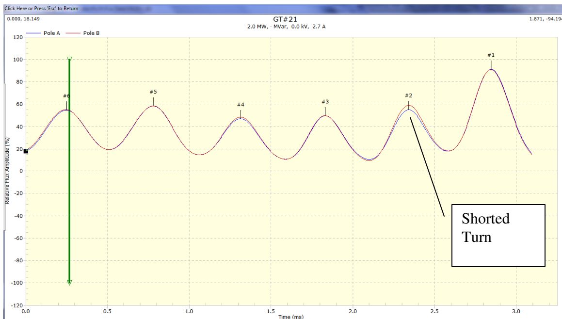
Fig 3: X-axis is time, Y-axis is normalized flux in percent. Plot shows comparison of the leading poles flux signals. FDZC is close to coil 6 (green line), short detected in coil 2
