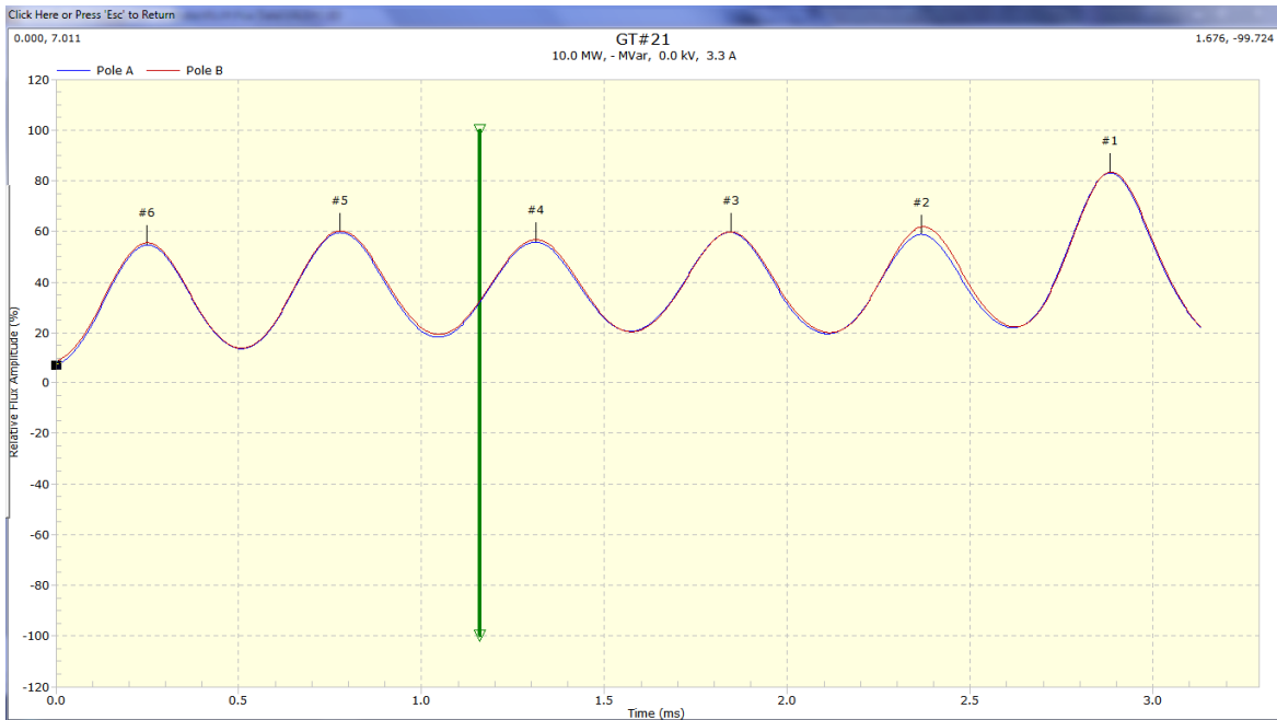
Fig. 4: X-axis is time, Y-axis is flux in percent. Pole A to pole B comparison, 10 MW load test
