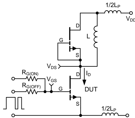
Figure 12: GS66516B switching time test circuit and waveforms
