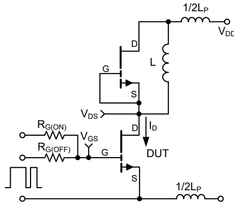
Figure 12: GS66516T switching time test circuit and waveforms
