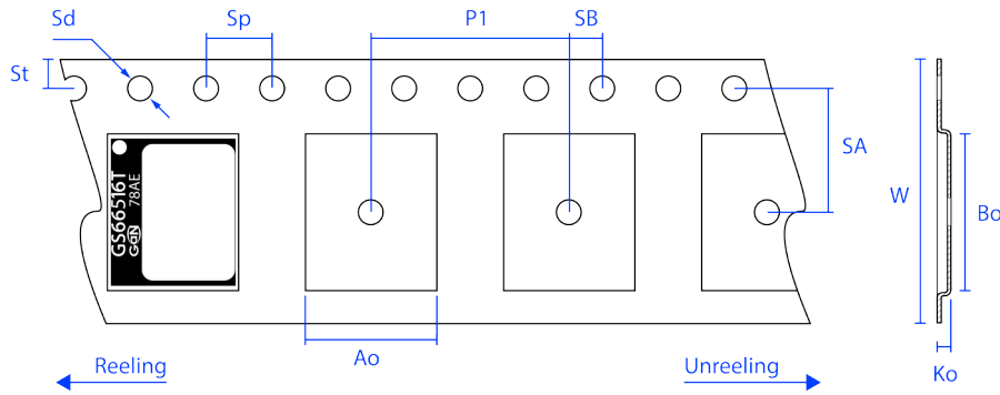
Dimensions (mm)
