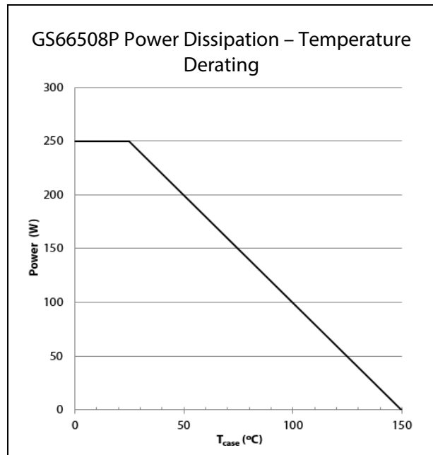
Figure 15: Power Derating vs. T_{case}
