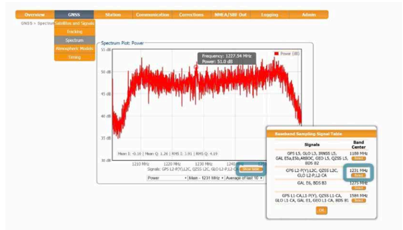
Figure 7 – Visualising RF interference – the spectrum view plot
