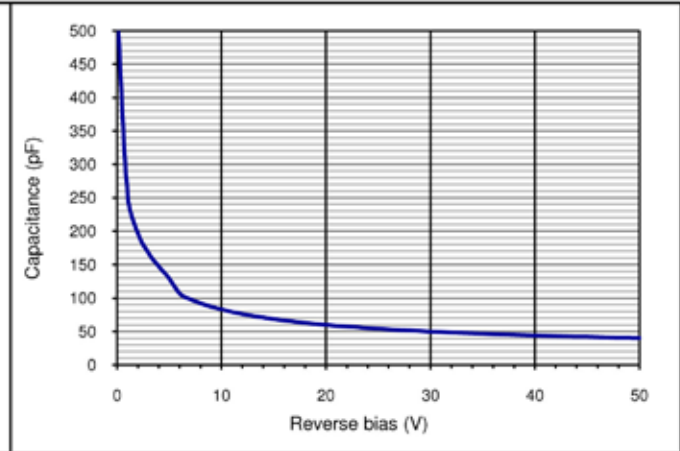
Capacitance as fct of reverse bias (23 °C)
