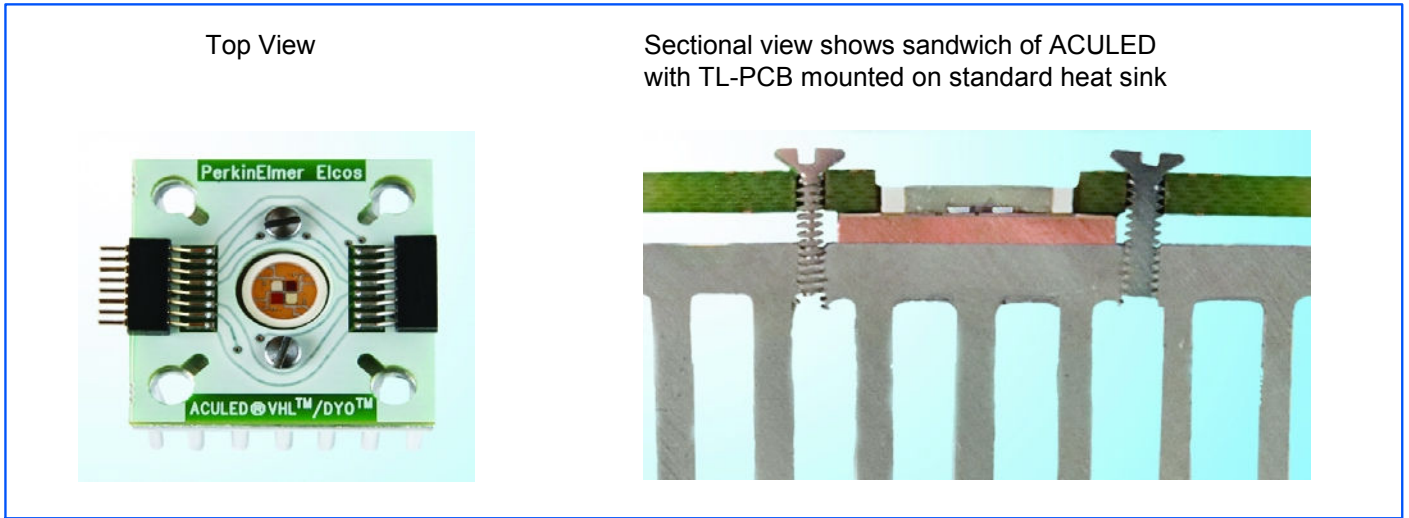
Figure 7. The Principle of TL-Mounting of the ACULED for Easiest Heat Management
