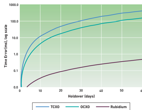
Plot of time error in milliseconds accumulated during holdover for different oscillator types. Note log scale of Y-axis.
